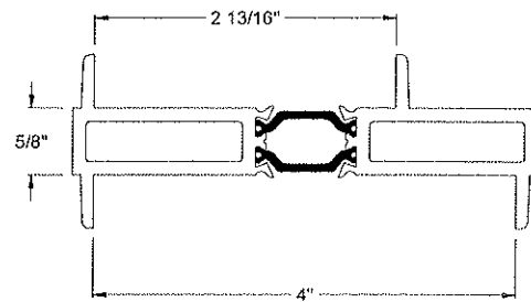
IF-1010 3 1/4" TO 4 3/8" TRANSITION STACK MULLION (MALE)
