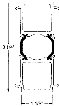
IF-0118 3 1/4" MULLION
