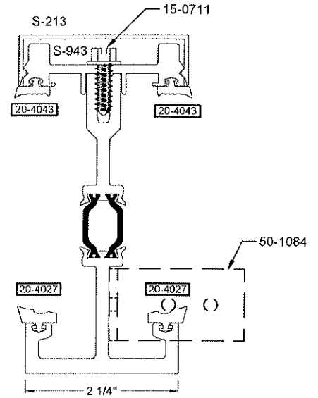
IF-1017 3 1/4" NX H.D. MULLION
