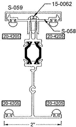
IF-1016 3 1/4" NX PRE-SET PANNING MULLION
