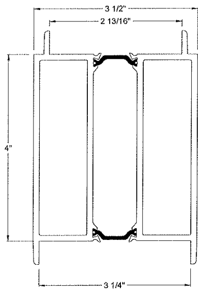
IF-1009 3 1/4" STACK MULLION
