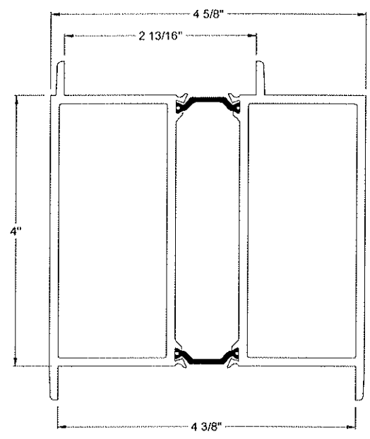
IF-1006 3 1/4" TO 4 3/8" TRANSITION STACK MULLION
