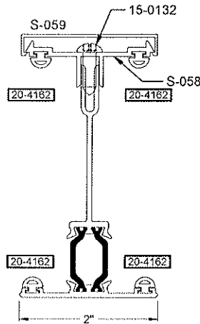
IF-1002 3 1/4" NX 3 PC. MULLION
