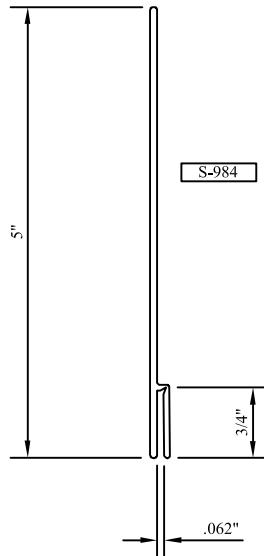
5" EXPANDER S-984
