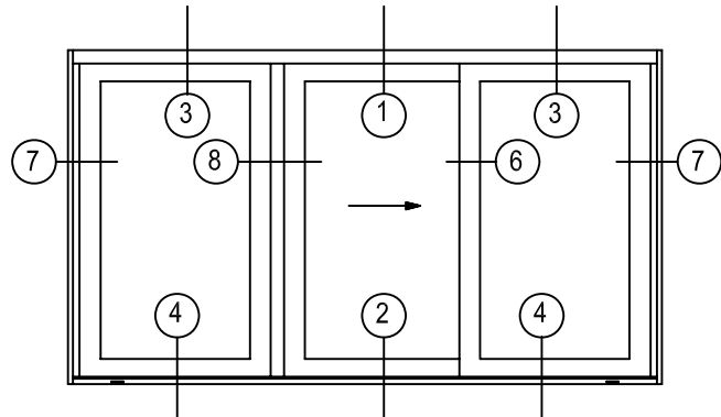
TR-840 (3 PANEL) (OXO ONLY) SLIDE RIGHT SHOWN (SPECIFY SLIDE DIRECTION)
