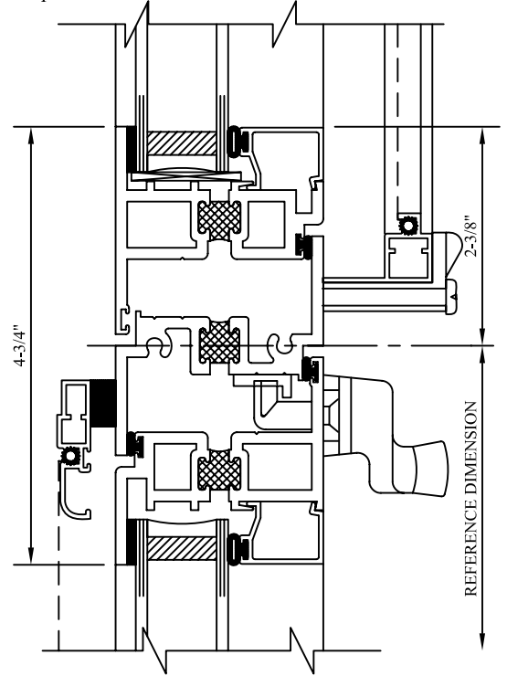
23 HORZ. INTEGRAL MULLION VENT OUT/VENT IN
