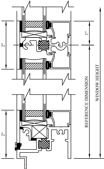
25 TR-2800 HORZ. INTEGRAL MULLION
