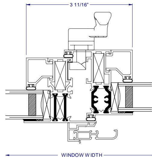
⑧ VERTICAL INTEGRAL MULLION (FIXED/VENT)
