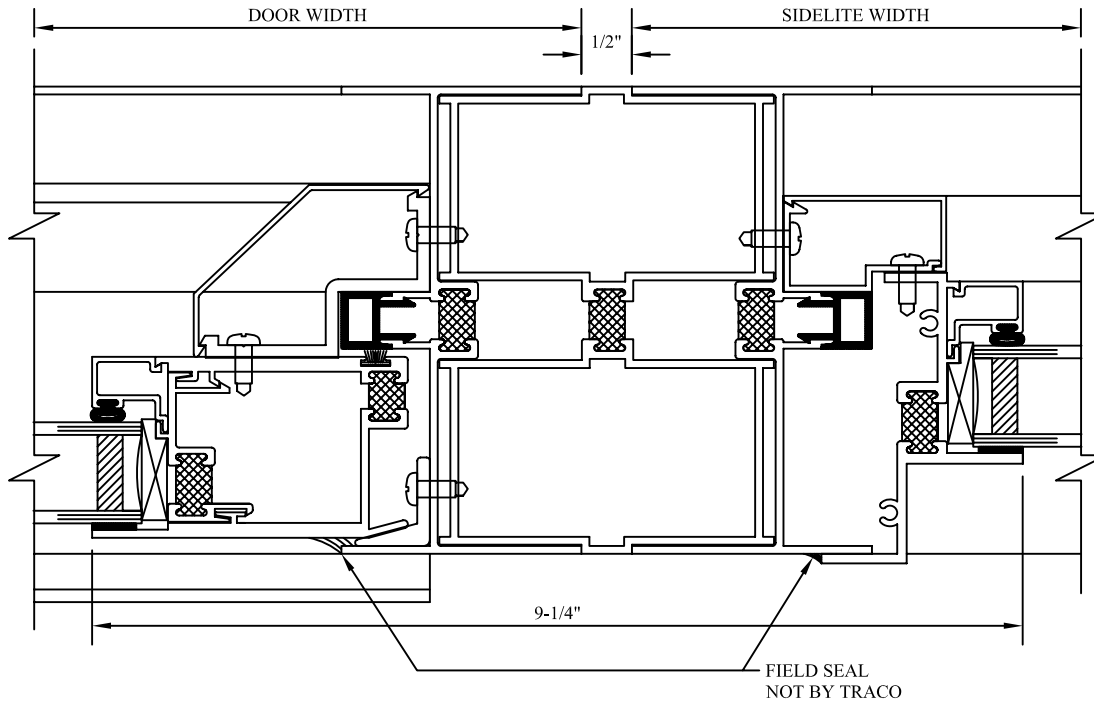
⑭ VERTICAL MULLION (FIXED/SIDELITE)
