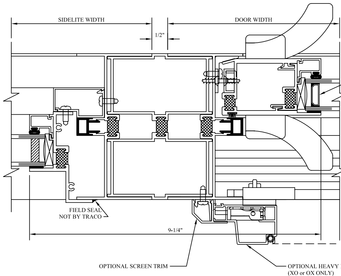
⑮ VERTICAL MULLION (SIDELITE/OPERATING)
