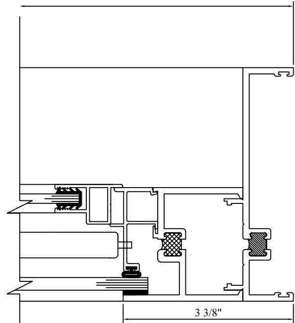
10 VENT JAMB (DUAL GLAZED) WINDOW WIDTH
