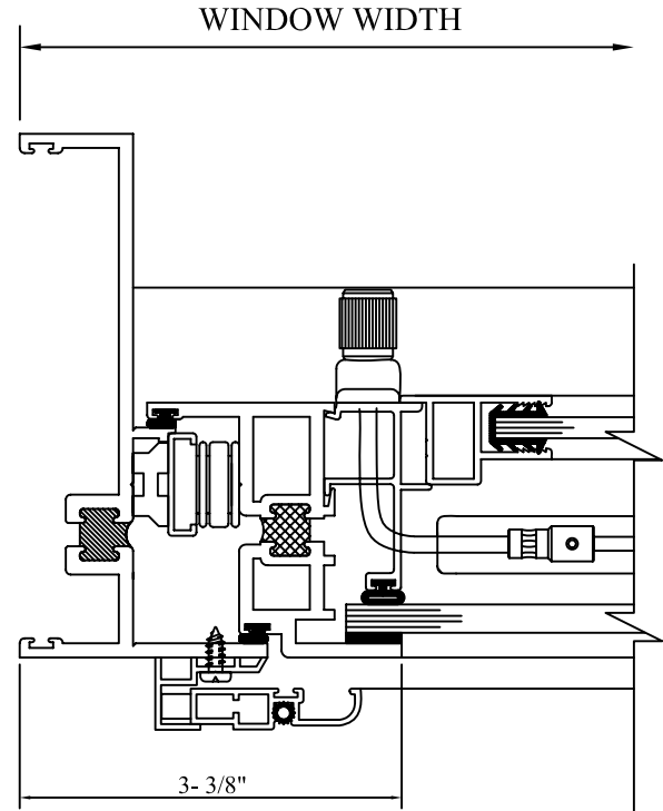
10 VENT JAMB (DUAL GLAZED) WINDOW WIDTH
