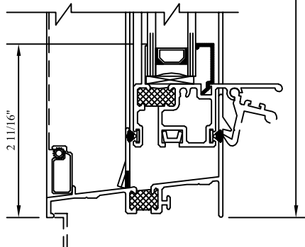
③ SILL
