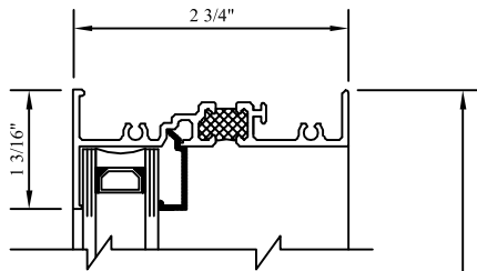
① HEAD
